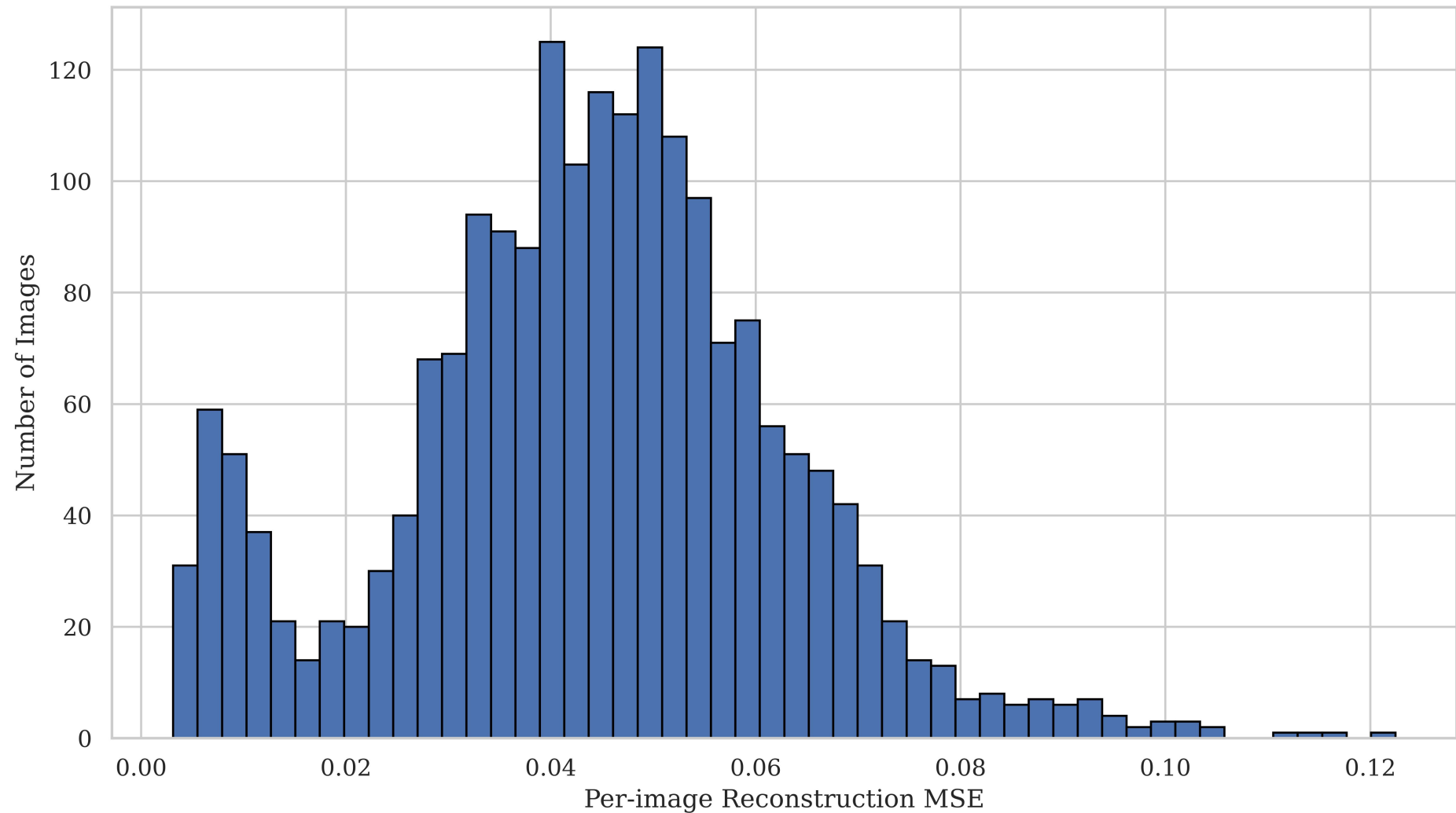
VAE Reconstruction Error Distribution
